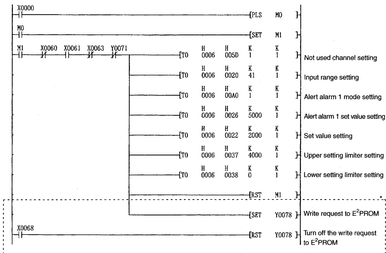
(b) Unused channel, input range, alert alarm 1, and set value, upper/lower setting limiter setting
