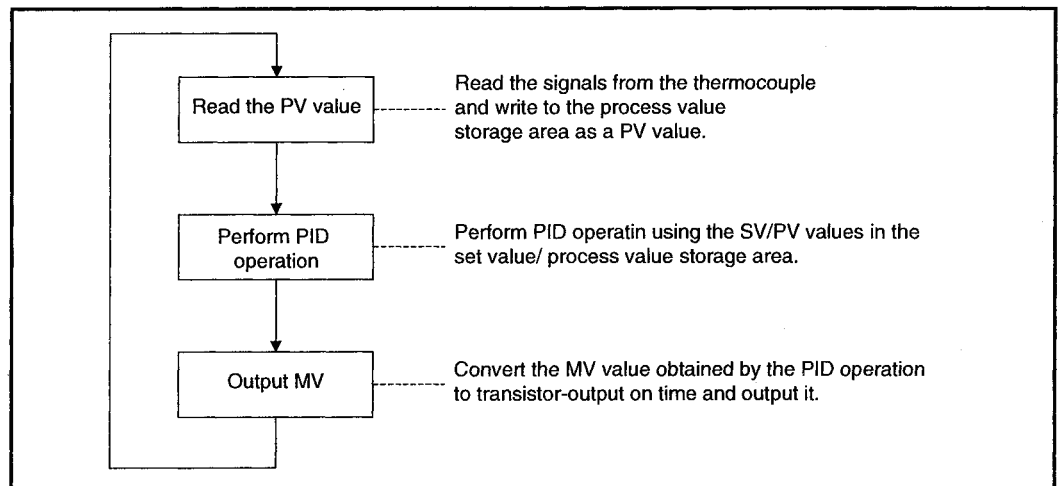
Fig. 1.4 PID control procedure
