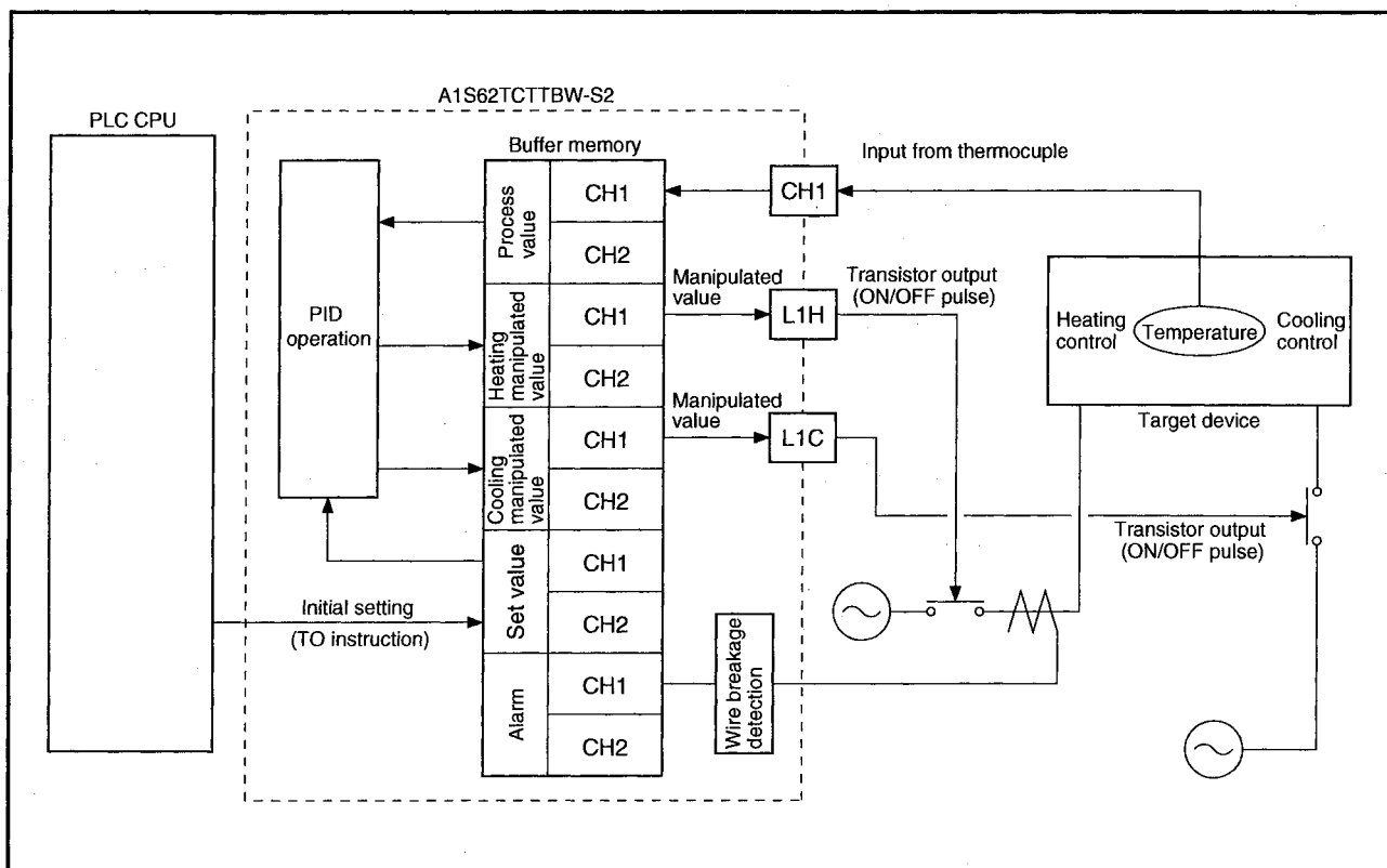
Fig. 1.2 A1S62TCTTBW-S2 processing overview
