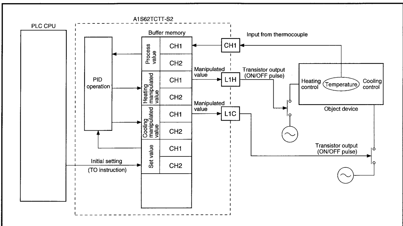
Fig. 1.1 A1S62TCTT-S2 processing overview
